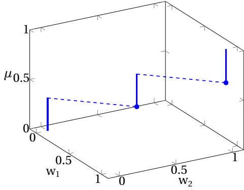
Figure (a) The payoff function w .
