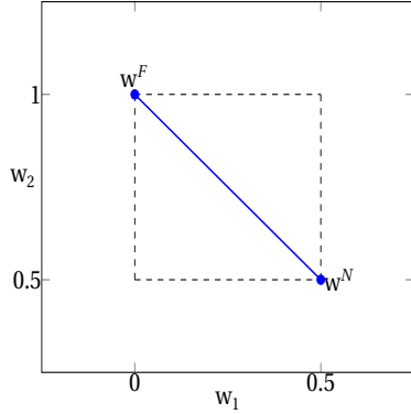
Figure (a) N = 2 and \rho = (0, 1)
