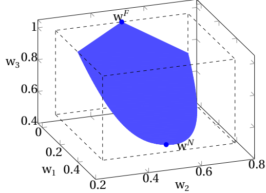
Figure (b) N = 3 and \rho = (0, 0.5, 1)
