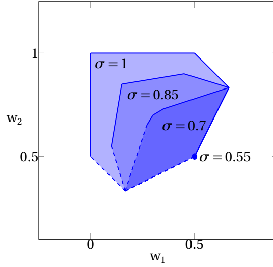
Figure 6: IP-set for different values of \sigma \in \{0.55, 0.7, 0.85, 1\} .
