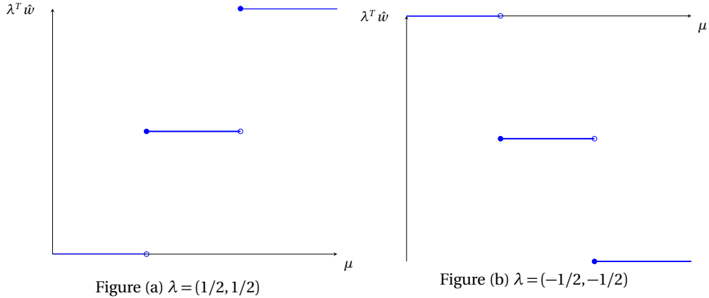
Figure 3: Objective function in Equation 8 for Example 1
