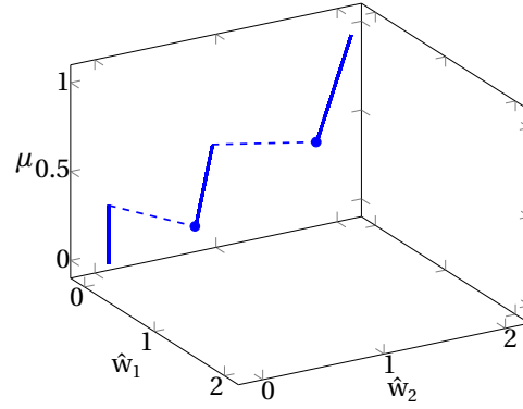
Figure (b) The adjusted payoff function \hat{w} .
