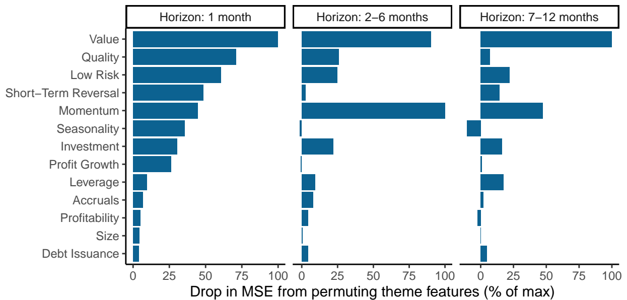
Figure C.3: Feature Importance across Return Horizons
