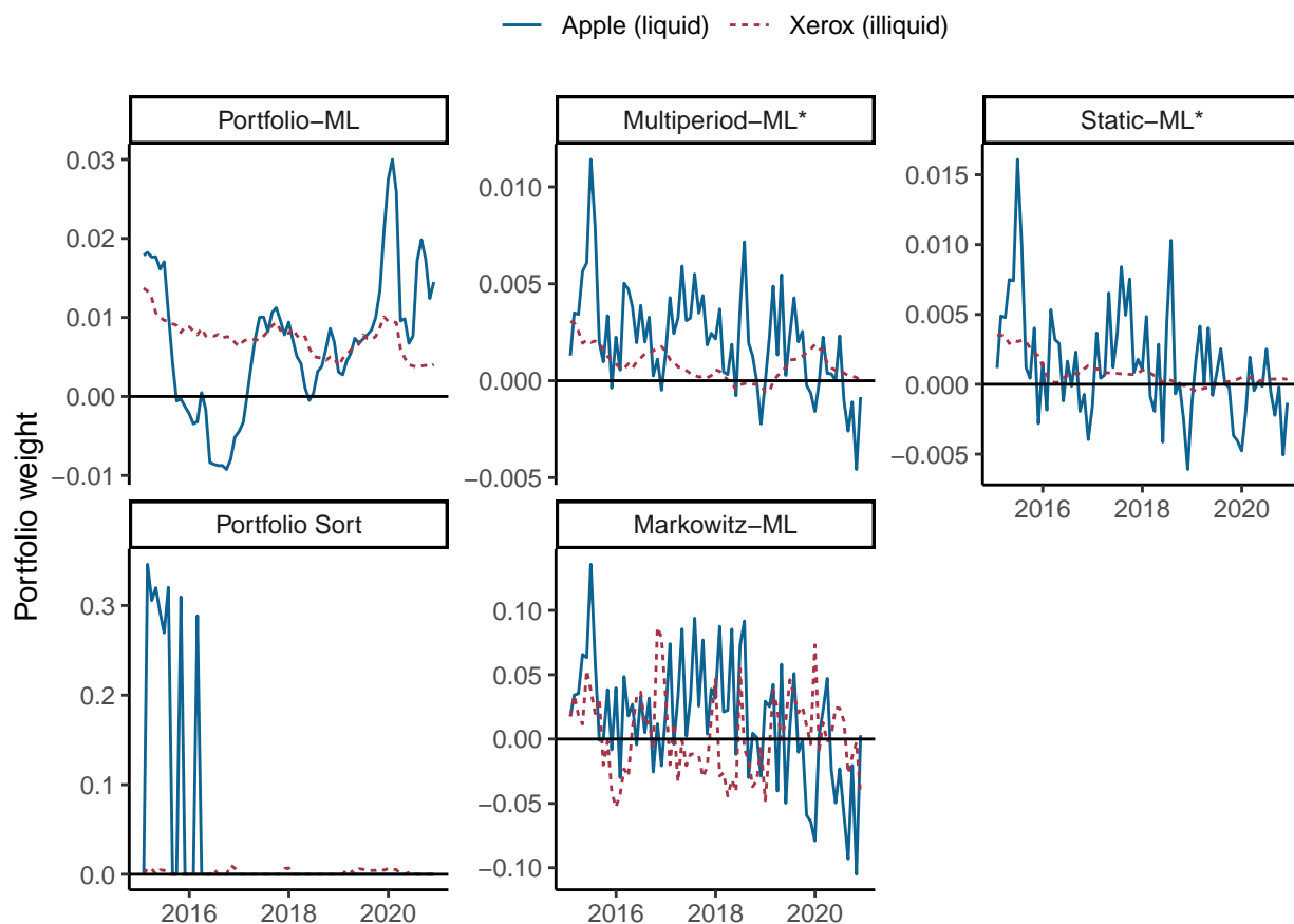
Figure 4: Portfolio Weights: Apple vs. Xerox
