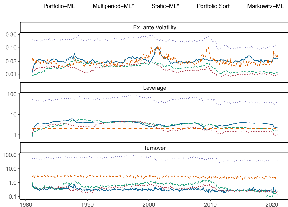
Figure 3: Portfolio Statistics over Time
