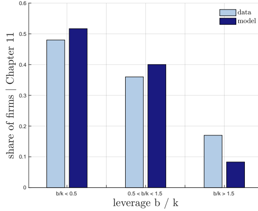
(a) Leverage ( b'/k' ) model and data
