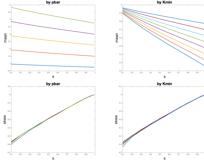
Figure 10: Uniform Distribution - Simulations
