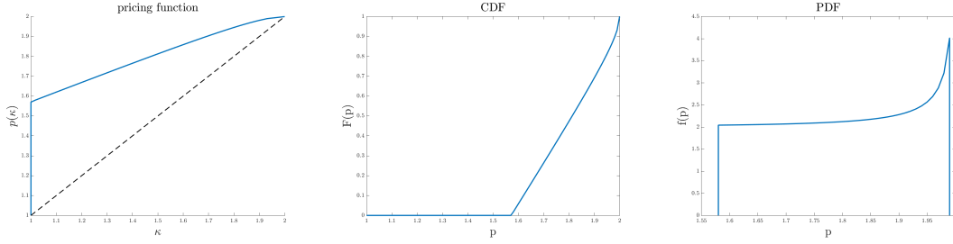
Figure 9: Uniform Distribution - Example
